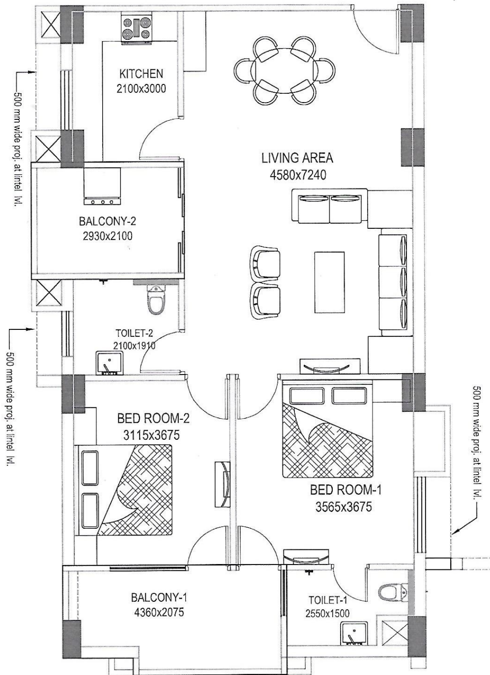
UNIT PLAN (TYPE-II)
