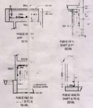
TYPICAL PUBLIC HEALTH SHAF T DETAILS (SCAL E : 1:40)
